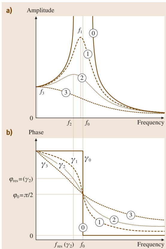
Fig. 16.4 (a) Resonance curve with no damping (0), and increasing damping (1)–(3). The undamped curve with resonance frequency f_0 exhibits a very high amplitude, whereas the resonance peak amplitude decreases with damping. This also involves a shift in resonance frequencies from f_1 to f_3 to lower values. (b) Corresponding phase curves showing no damping (0), and increasing damping (1)–(3). The step-like phase jump at resonance of the undamped resonance gradually broadens with increasing damping
