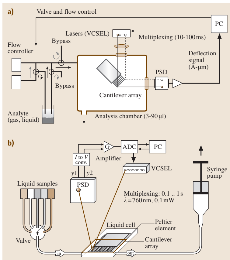
Fig. 16.6 Schematic of measurement set-ups for (a) a gaseous (artificial nose) and (b) a liquid environment (biochemical sensor)
