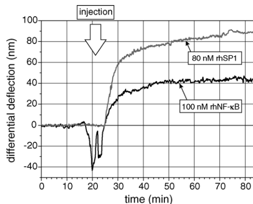
Fig. 5. Comparison of rhNF-κB with rhSP1. Differential signal of experiments conducted by injection of 100 nM rhNF-κB or 80 nM rhSP1 to two different cantilever arrays. For rhNF-κB, cantilevers functionalized with SP1-binding oligonucleotides were used as reference. Cantilevers functionalized with the rhNF-κB-binding oligonucleotides served as references when rhSP1 was injected.
