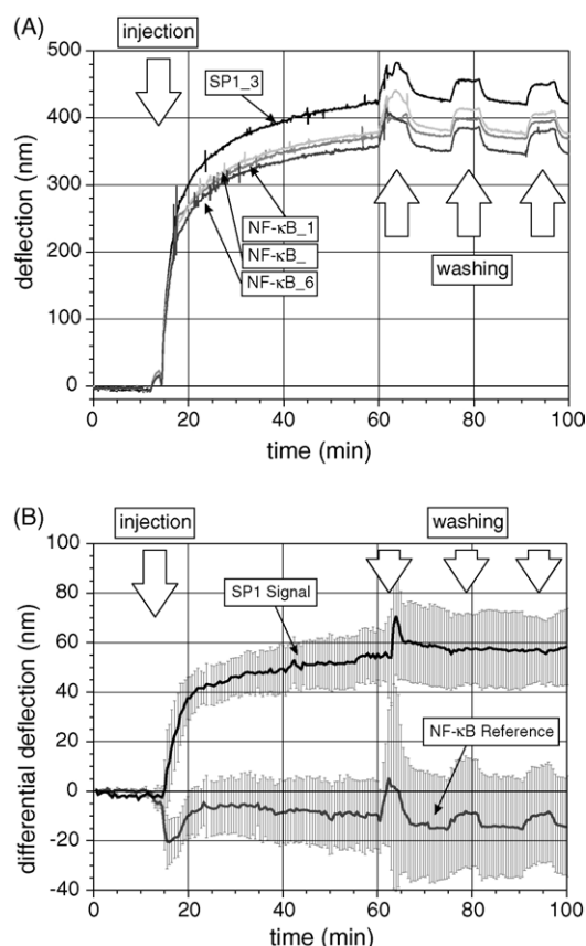
Fig. 4. Representation of raw data from an experiment in which 80 nM of rhSP1 is injected. (A) The bending curves of cantilever 3 (SP1_3), functionalized with SP1-binding oligonucleotides and three reference cantilevers (NF-κB_1, NF-κB_4, and NF-κB_6) functionalized with NF-κB-binding oligonucleotides. For clarity only four representative curves are displayed. Other cantilevers of the same array exhibited the same behavior. Comparison of averages and standard deviations of 3 SP1 signals with 3 NF-κB references. (B) Average differential SP1 signal obtained from differences in the responses of cantilever 3 and of cantilever 1 (SP1_3–NF-κB_1), cantilever 4 (SP1_3–NF-κB_4), and cantilever 6 (SP1_3–NF-κB_6). Average differential NF-κB reference signal calculated from differences in the responses of cantilever 4 and of cantilever 1 (NF-κB_4–NF-κB_1), cantilever 6 (NF-κB_4–NF-κB_6), cantilevers 6 and 1 (NF-κB_6–NF-κB_1).
