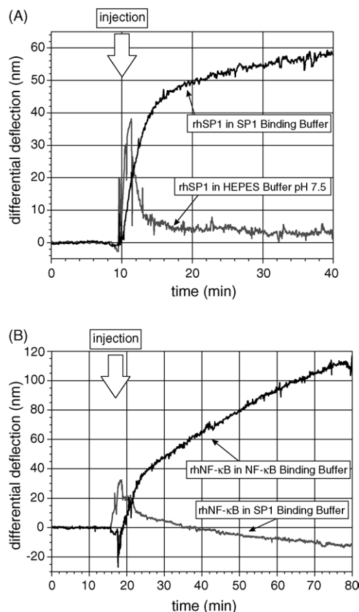
Fig. 3. Investigation of buffer conditions for binding the transcription factor rhSP1. (A) 200 \mu l 80 nM of rhSP1 was injected. Initially very simple buffer conditions were chosen (20 mM HEPES, pH 7.5). In subsequent experiments, we found that optimized conditions promote binding of rhSP1 (SP1-binding buffer: 20 mM HEPES pH 7.5, 0.1% Tween 20, 5 \mu M ZnSO 4 , 6 mM MgCl 2 , 50 mM KCl, 50 mM NaCl). Optimizing binding conditions for rhNF- \kappa B. (B) 200 \mu l 400 nM rhNF- \kappa B was injected. rhNF- \kappa B required a different buffer (NF- \kappa B-binding buffer: 10 mM HEPES pH 7.9, 50 mM KCl, 0.05% NP40, 10% glycerol).
