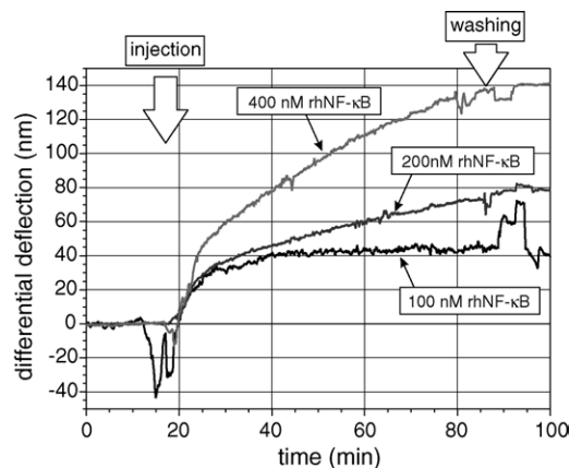
Fig. 6. Differential signals obtained by injection of three different rhNF- \kappa B concentrations (100, 200 and 400 nM).
