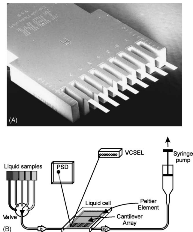
Fig. 1. (A) SEM image of a microfabricated cantilever array. A cantilever is 500 \mu\text{m} long, 100 \mu\text{m} wide and 500 nm thick. The pitch distance from the middle of one cantilever to the middle of the next is 250 \mu\text{m} . The cantilevers are coated with 2 nm of Ti and 20 nm of Au on top. The Au layer serves as a substrate to functionalize the cantilevers with thiol-modified oligonucleotides on one side. (B) The cantilever array is placed inside a liquid filled cell having a volume of 50 \mu\text{l} . Different samples can be injected using a syringe pump and a five-fold valve. A Peltier element placed below the liquid cell serves to assess the thermal and mechanical properties of the cantilevers. Cantilever bending is detected by laser beam deflection using a time-multiplexed vertical-cavity surface-emitting laser (VCSEL) array and a position-sensitive detector (PSD).
